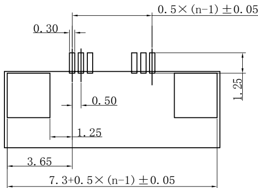
PCB BOARD LAYOUT
