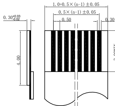
RECOMMENDED FPC/FFC DIM
